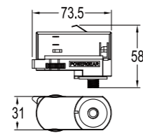
3-PHASE 0440S
