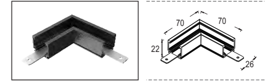
L Joint(R)
