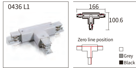
"T" connector "left I"
