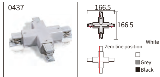
"+" connector
