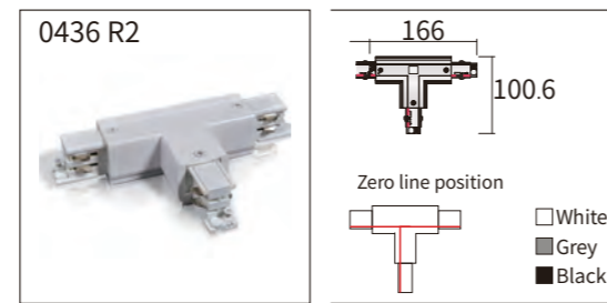
"T" connector "right II"
