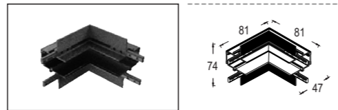
L Joint
