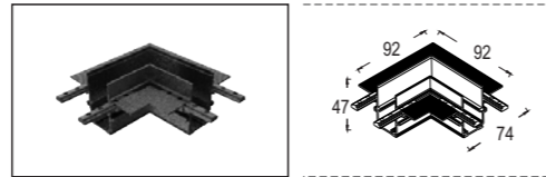
L Joint(R)
