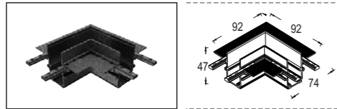
L Joint(L)
