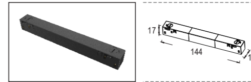
I Joint
