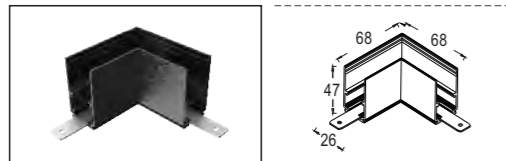
L Joint(L)
