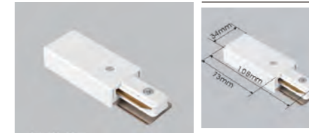
Feeder
