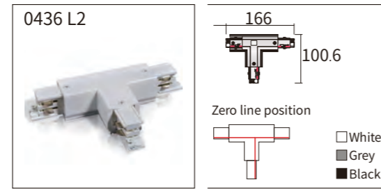
"T" connector "left II"
