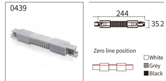
Soft connector
