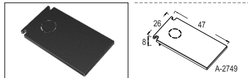
End Cover
