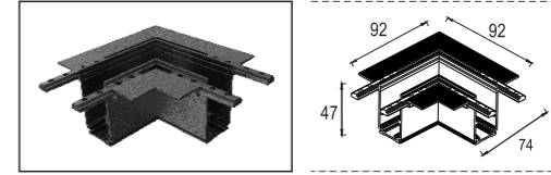
L Joint(R)
