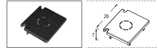
End Cover
